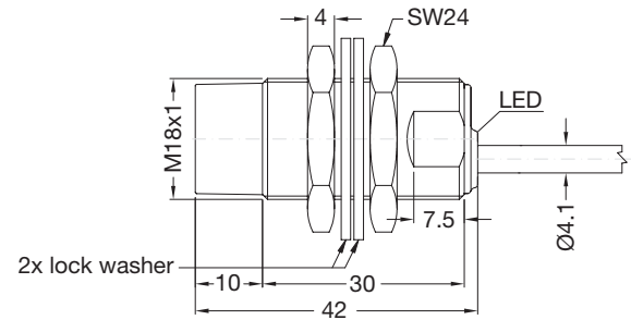
Fig. 22 Short body, non-flush version, cable
