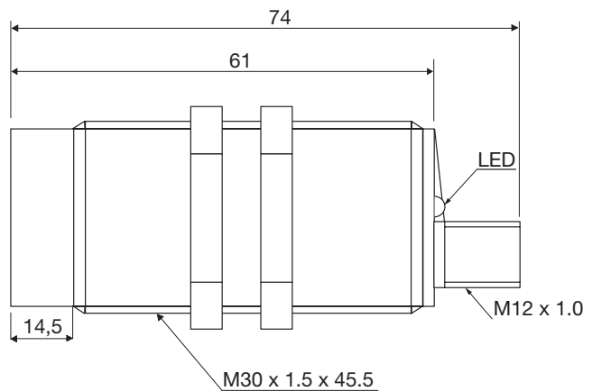
Fig. 9 Plug CA30CAN...M1IO
