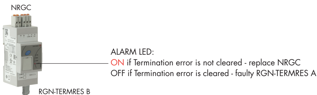
Fig. 7.3: NRGC terminated with RGN-TERMRES B
