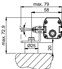
Angled fixing bracket + Orientable support + Antivibration support
