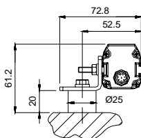
Angled fixing bracket + Orientable support
