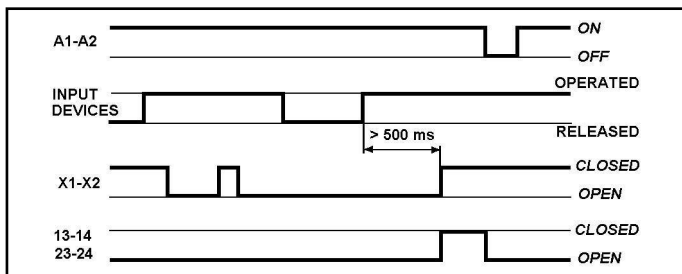
Fig. 8: NSC02DB - Diagramma funzionale / Functional diagram (mod. "SC" e / and "DC")
