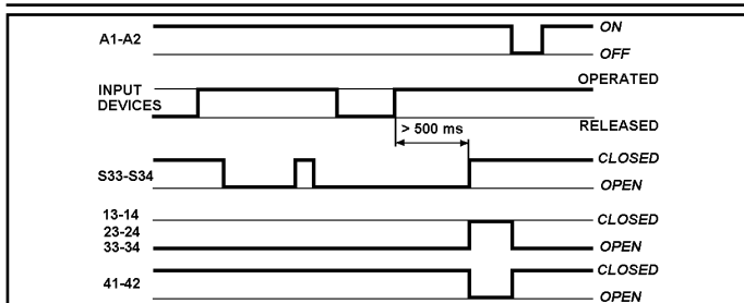
Fig. 7: NSC13DB - Diagramma funzionale / Functional diagram (mod. "SC" e / and "DC")
