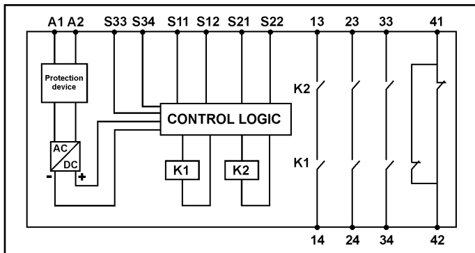
Fig. 1 - Schema circuitale dei moduli NSC13D / NSC13D circuit diagram
