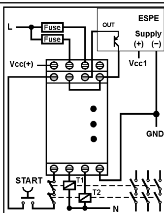
Fig. 9: ESPE 1 uscita PNP a 2 fili / One 2-wires PNP output
