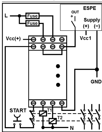
Fig. 6 ESPE: 1 uscita a relè a 1 filo / One 1-wire relay output
