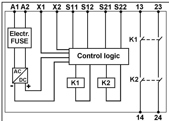
Fig. 1 - Schema circuitale dei moduli NLG02D724 / NLG02D724 circuit diagram
