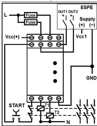
Fig. 4: ESPE: 2 uscite a relè a 1 filo / Two 1-wire relay outputs
