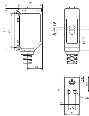
LD30ETB...M5IO
