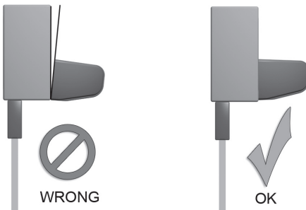
Fig. 4 Sensor alignment: The sensor must be mounted on a wall parallel to the door. The sensor can accept a deviation of +3 degrees.
