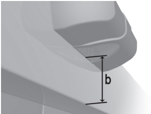
Fig. 4 Sensor alignment: The sensor must be mounted on a wall parallel to the door. The sensor can accept a deviation of +3 degrees.
