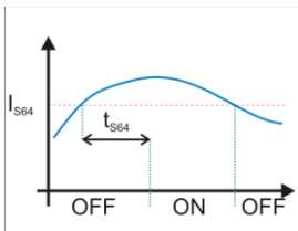
ANSI 64 delayed trip
