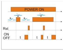
Timer function
