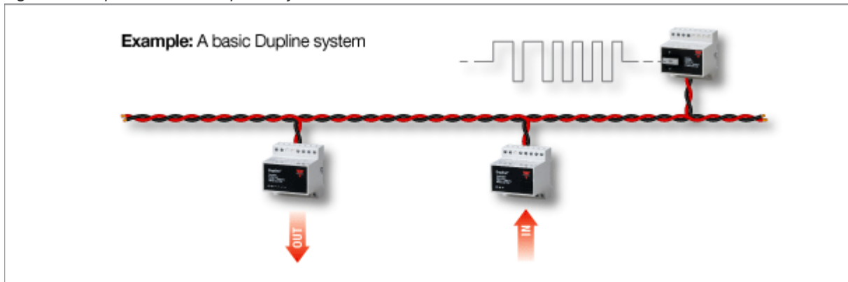
Fig. 16: Example of a basic Dupline® system
