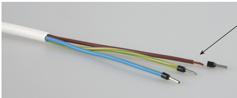
Fig. 31: 3 * 1,5 mm 2 multi-core wire with ferrule
