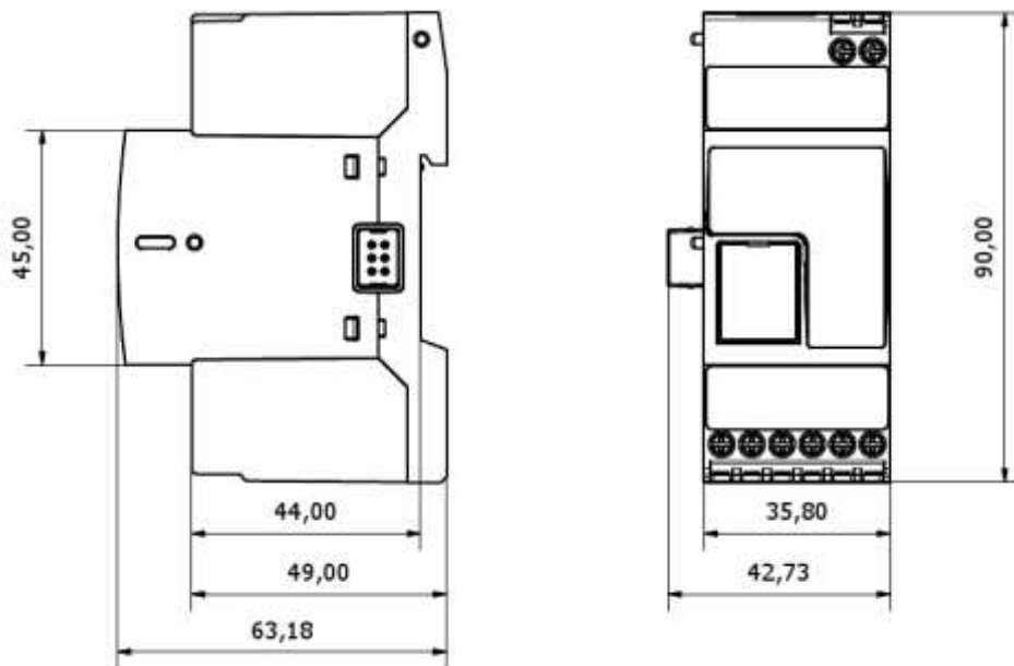
Dimensions Eos-Box
