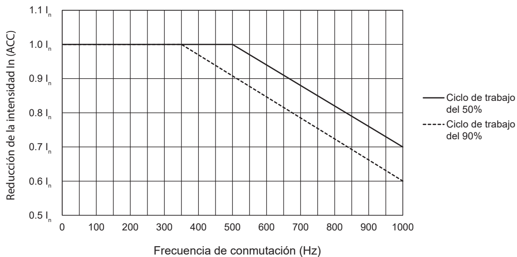
Fig. 4 Current derating vs. switching frequency
