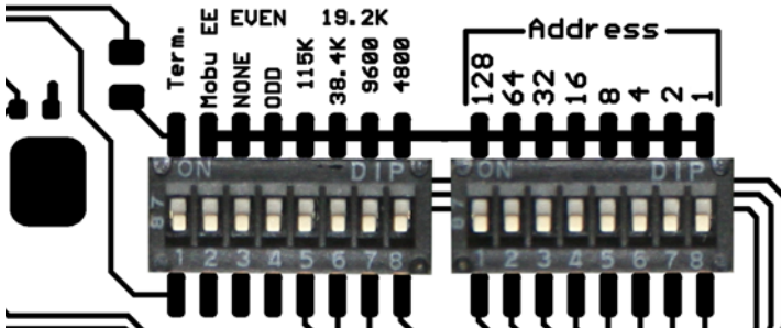
Fig. 10: detailed view DIP switches
