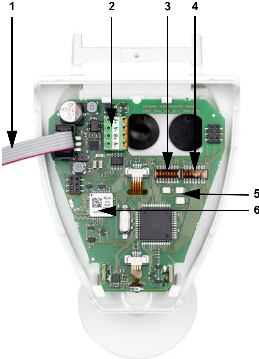
Fig. 9: Overview PCB
