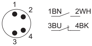
1NC + 1NO, Stecker
