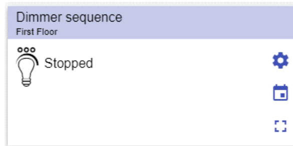
56. Dimmsequenz
